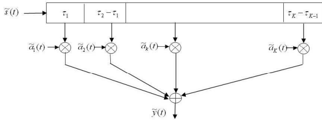
Fig. 1. Tapped-delay-line channel model with variable tap spacings.
