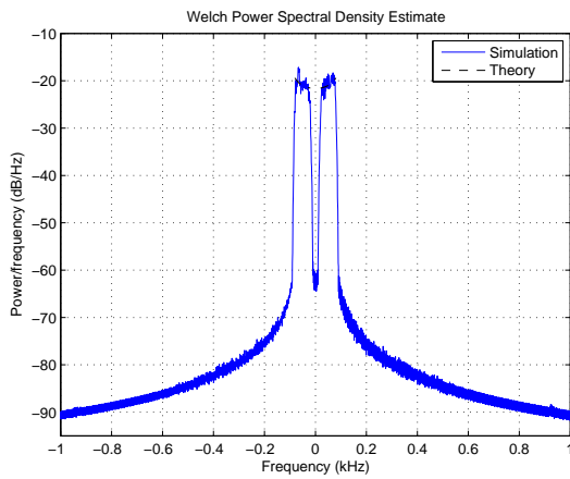
Fig. 15. Power spectrum of the complex fading process for a Rayleigh channel with a restricted Jakes Doppler spectrum, with f_{d,min} = 20 Hz and f_{d,max} = 80 Hz.
