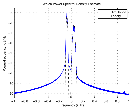
Fig. 21. Power spectrum of the complex fading process for a Rayleigh channel with a bi-Gaussian Doppler spectrum, with parameters corresponding to the COST 207 GAUS1 Doppler model.
