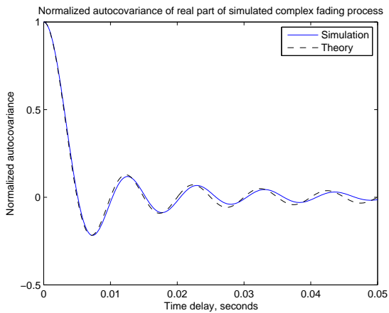
Fig. 10. Autocovariance (real part) of the complex fading process for a Rayleigh channel with a flat Doppler spectrum.
