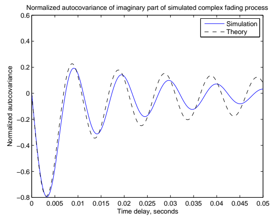
Fig. 17. Autocovariance (imaginary part) of the complex fading process for a Rayleigh channel with an assymetrical Jakes Doppler spectrum, with f_{d,min} = -100 Hz and f_{d,max} = 0 Hz.
