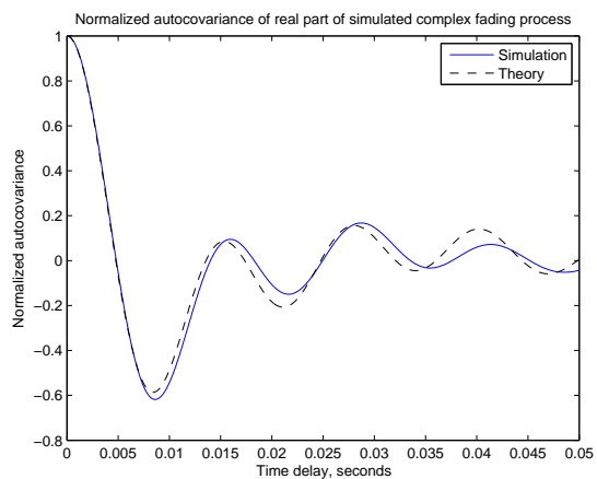
Fig. 14. Autocovariance (real part) of the complex fading process for a Rayleigh channel with a restricted Jakes Doppler spectrum, with f_{d,min} = 20 Hz and f_{d,max} = 80 Hz.
